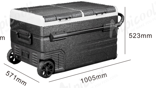
Model:TWW115 113 Quarts dual zone
