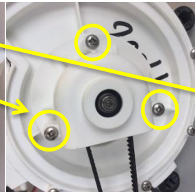
9. Remove screws
