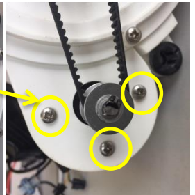
10. Remove screws
