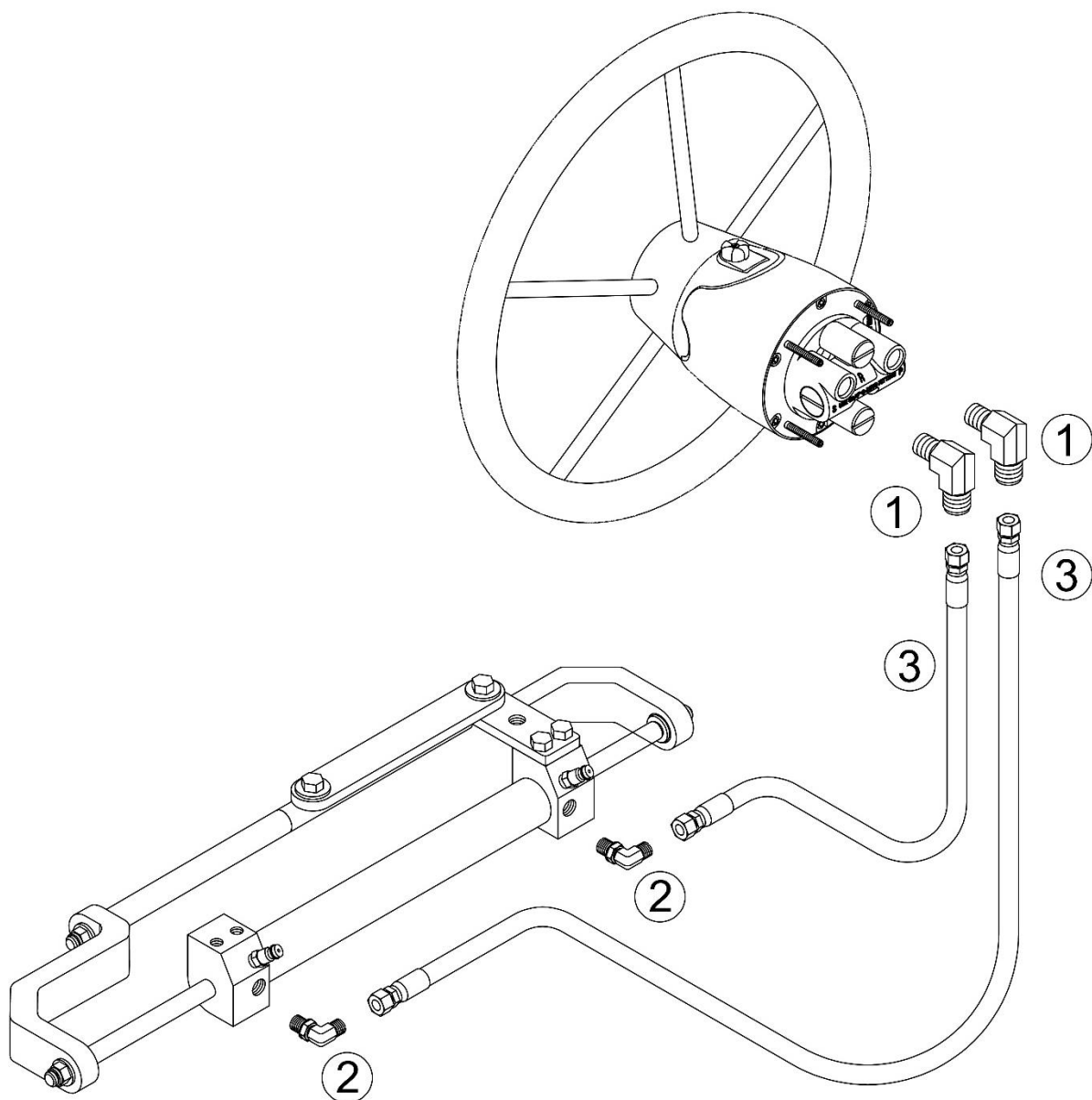
Fitting and Hoses For MO 100H
